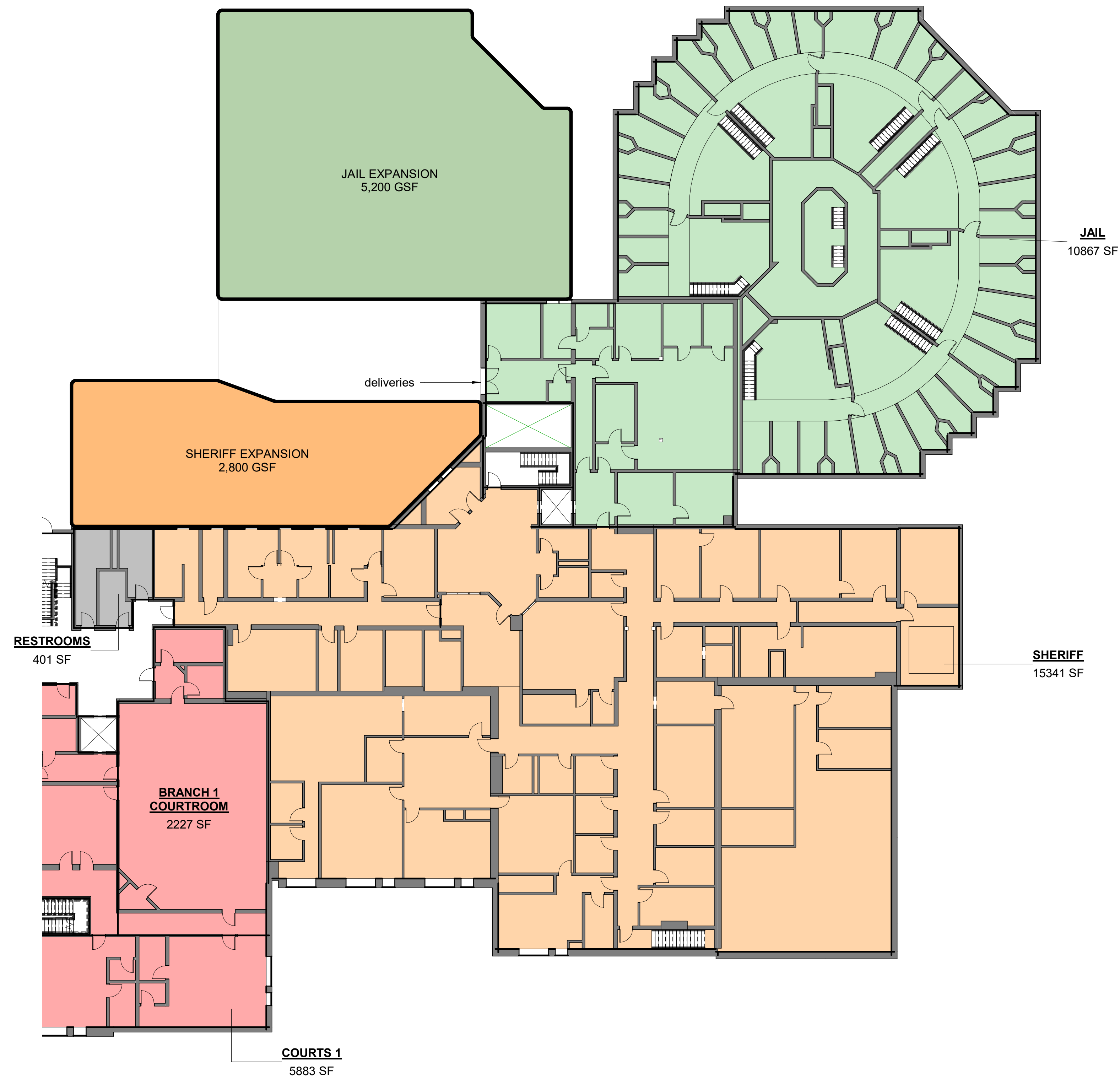
1 First Floor - Option 2 X103 1/16" = 1'-0"
